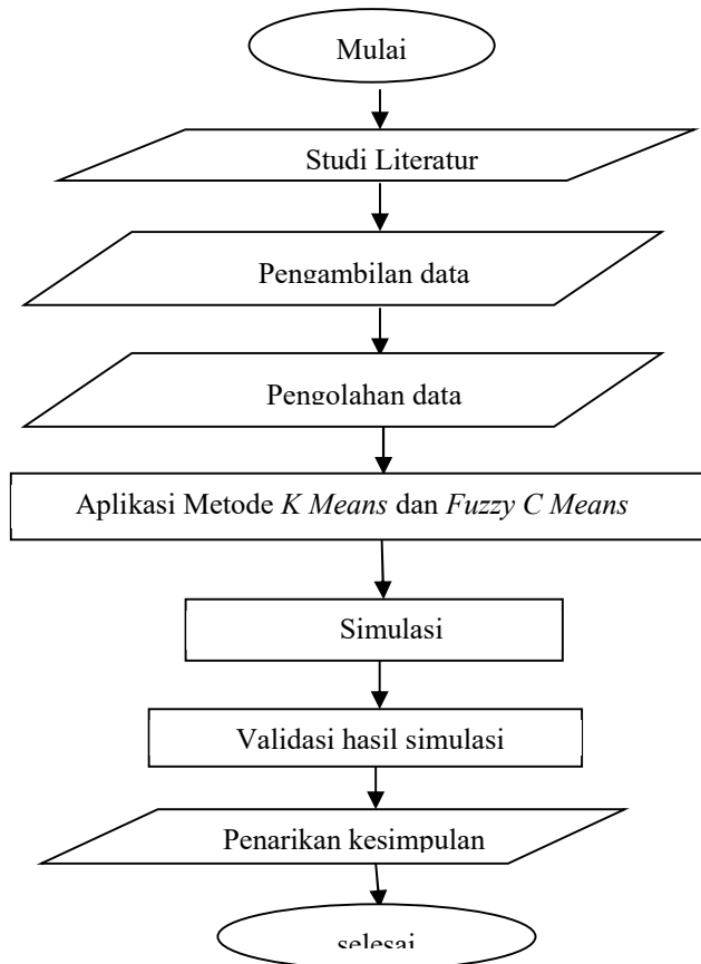
Gambar 1. Flowchart Penelitian
