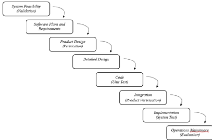
Gambar 1. Model Waterfall
